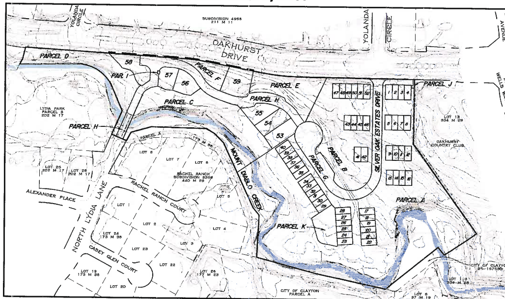
DEVELOPMENT PLAN & VESTING TENTATIVE MAP SCALE: 1"=100'
