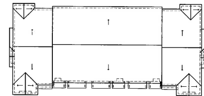
Roof Plan
