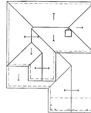
Roof Plan
