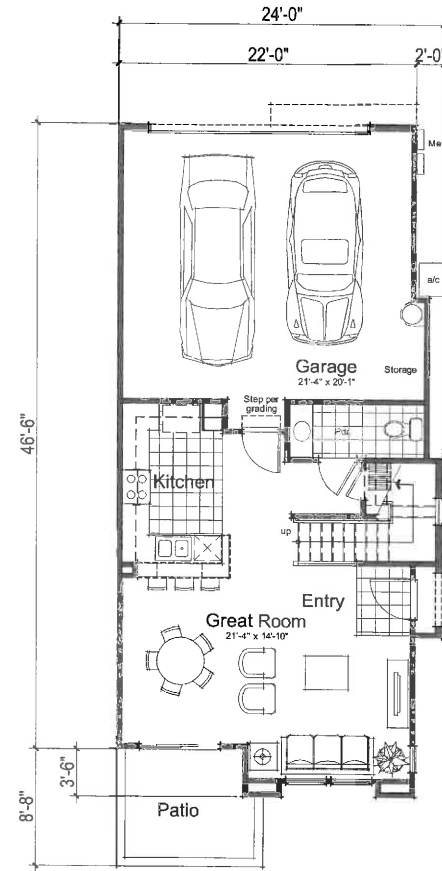
First Floor 613 Sq Ft
