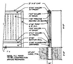
WOOD FENCE W/KICKBOARD SCALE: 1/2\"/>
