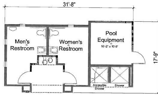
Cabana Floor Plan
