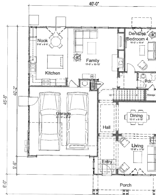
First Floor 1238 Sq Ft
