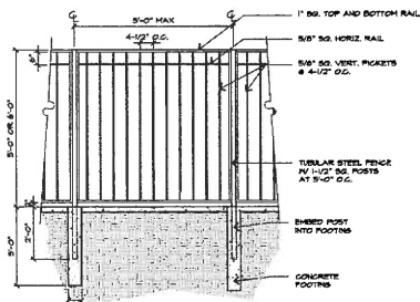
TUBULAR STEEL FENCE SCALE: 1/2\"/>
