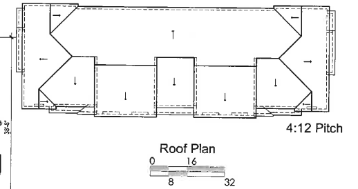
Building F - 6 Plex Tuck Under
