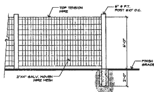
WIRE MESH FENCE SCALE: 3/8\"/>
