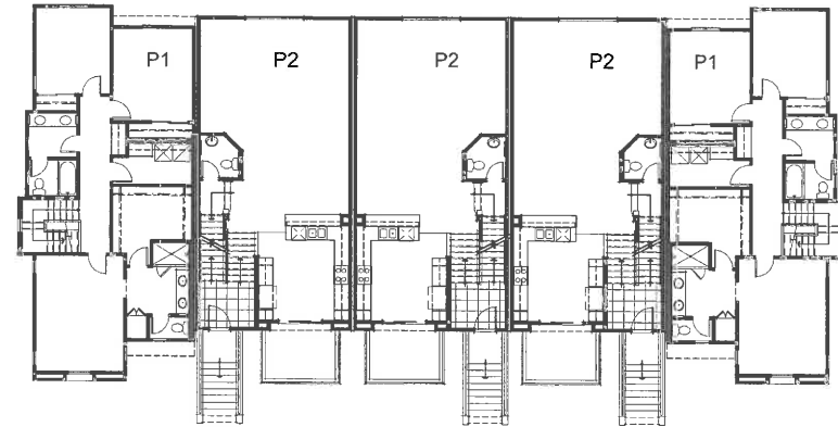
Second Floor
