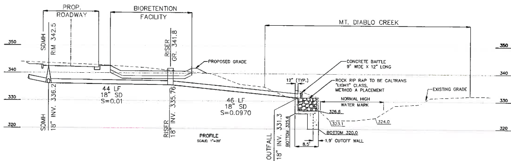
OUTFALL STRUCTURE DETAIL
