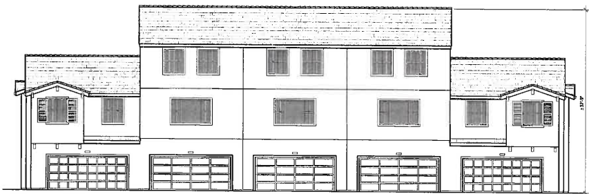
Rear Elevation
