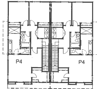
Third Floor
