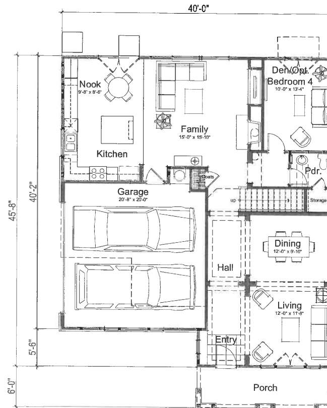
First Floor 1258 Sq Ft
