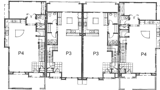
Second Floor
