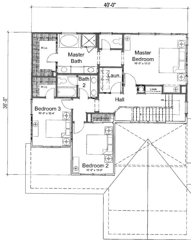
Second Floor 1054 Sq Ft
