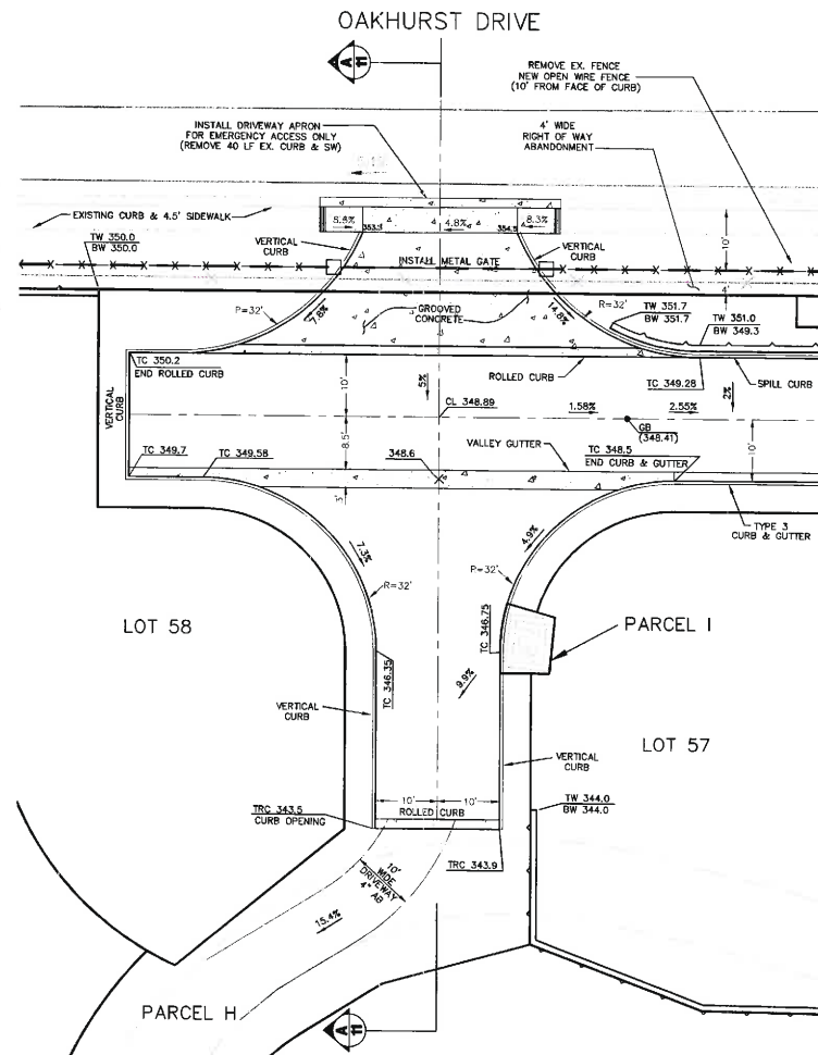
EMERGENCY VEHICLE ACCESS DETAIL
